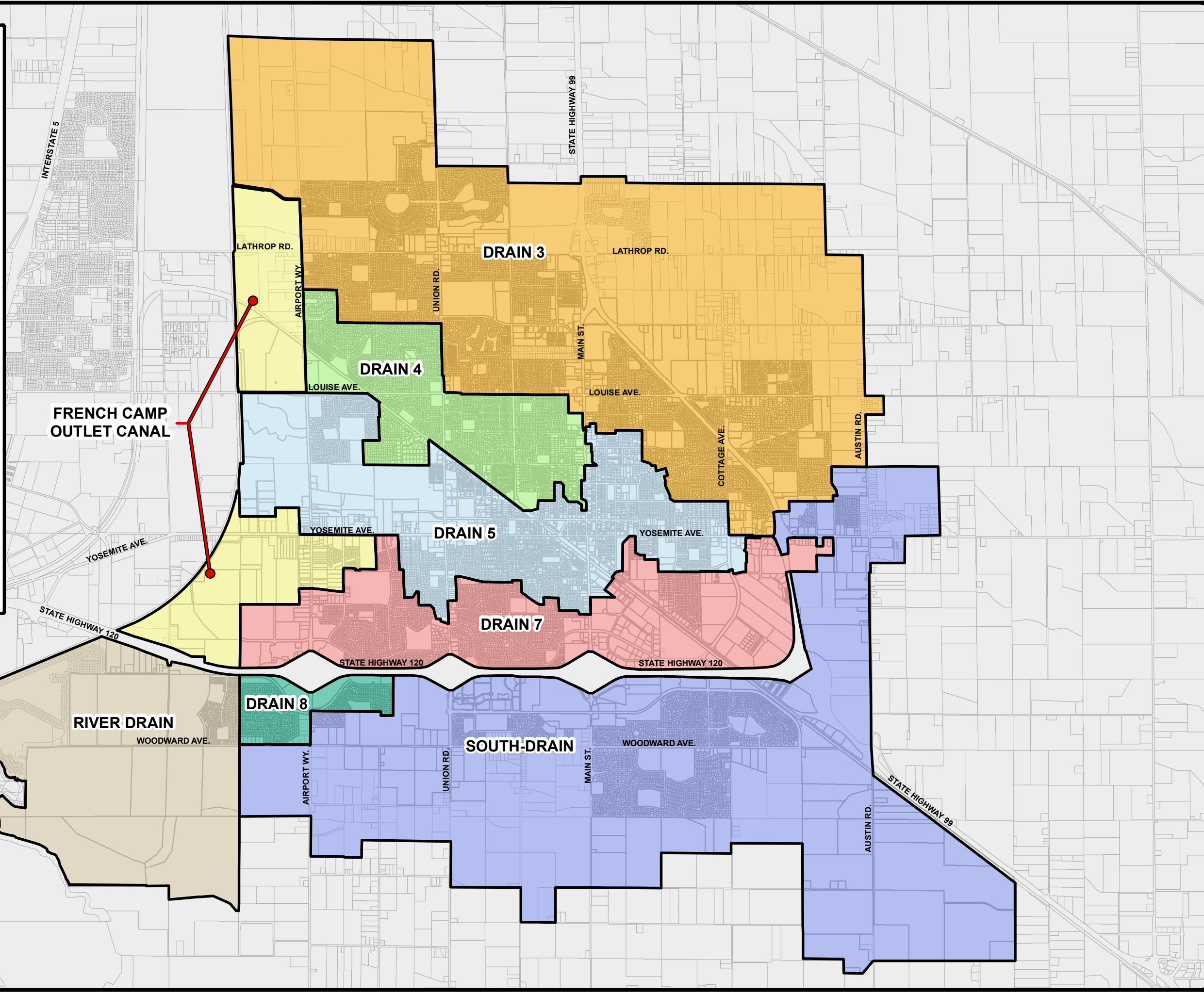
Figure 4-2 STORM DRAIN SHEDS
