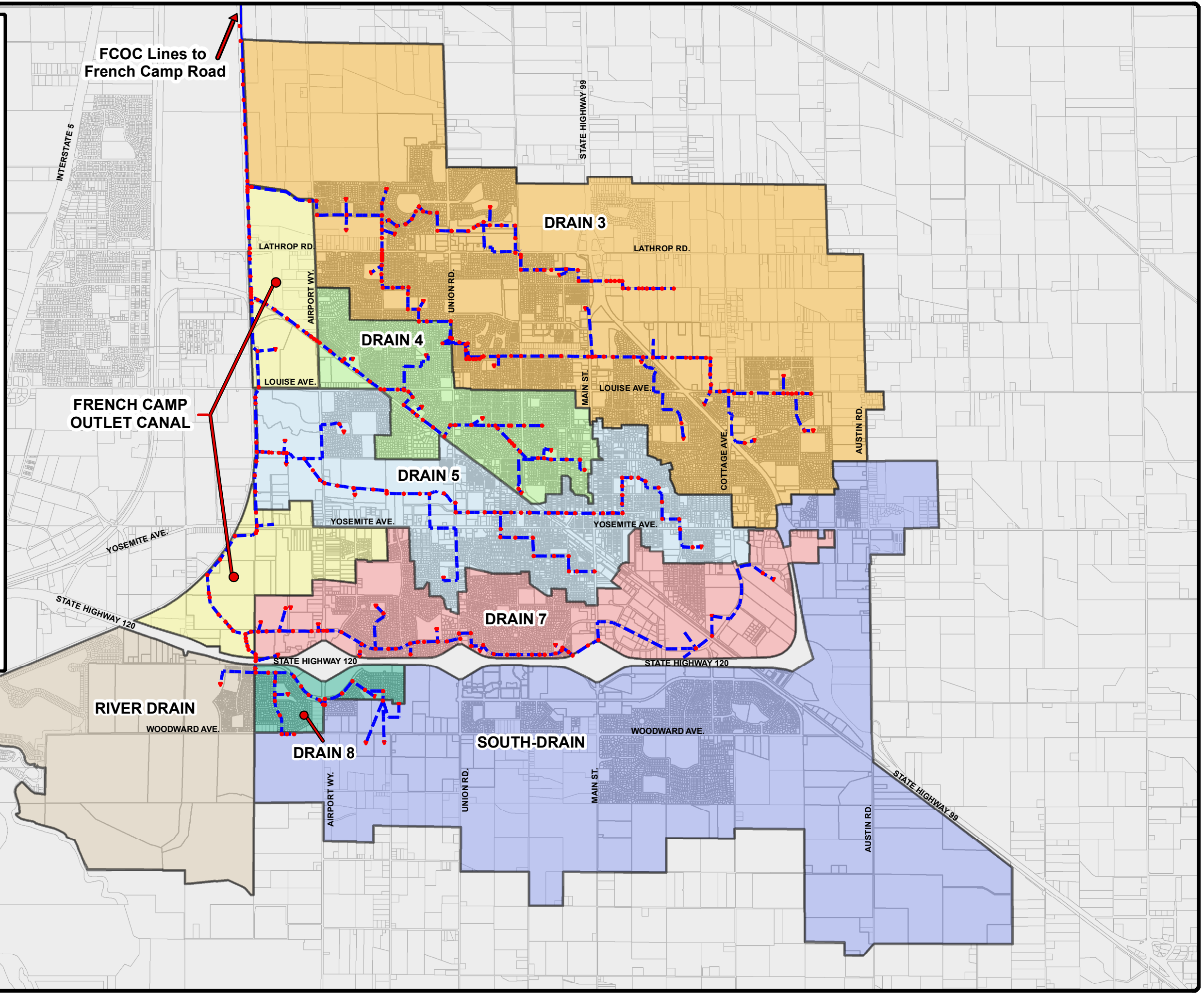
Figure 4-3 Schematic of XP-SWMM Model
